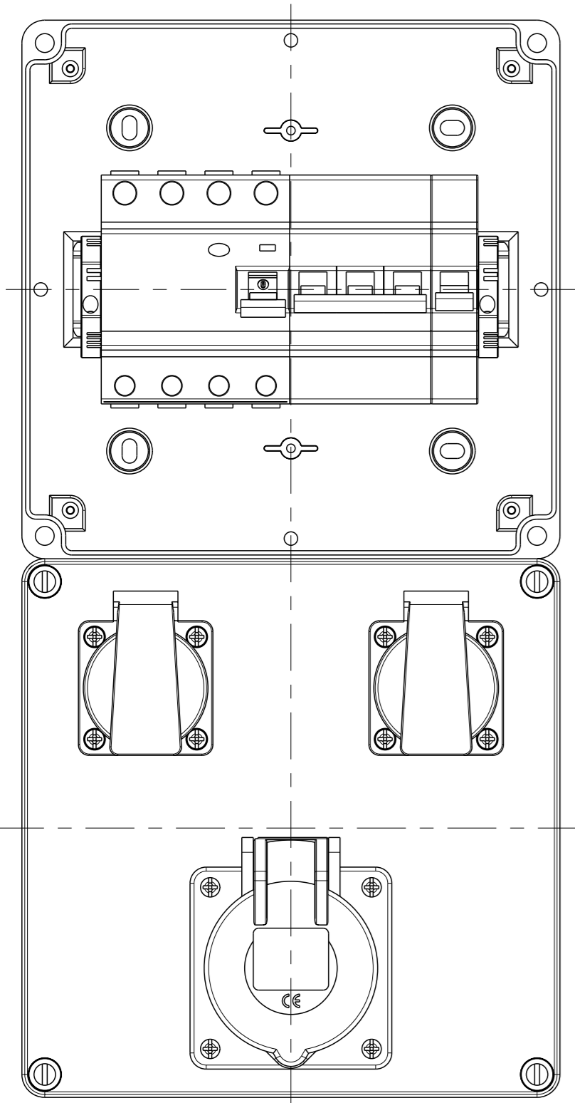
STV 912-K Innenansicht interior view
