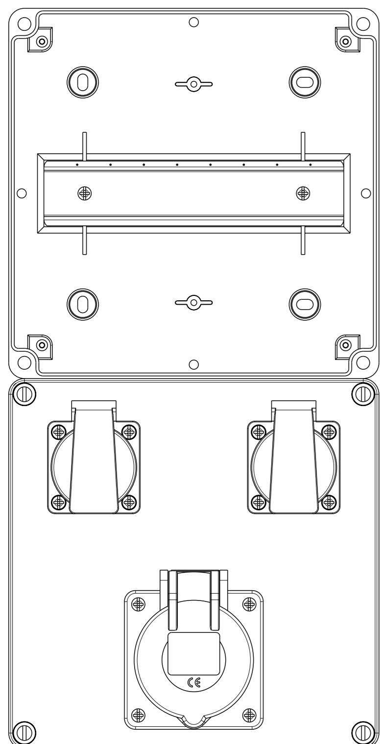
STV 912-S STV 912-S32 Innenansicht interior view
