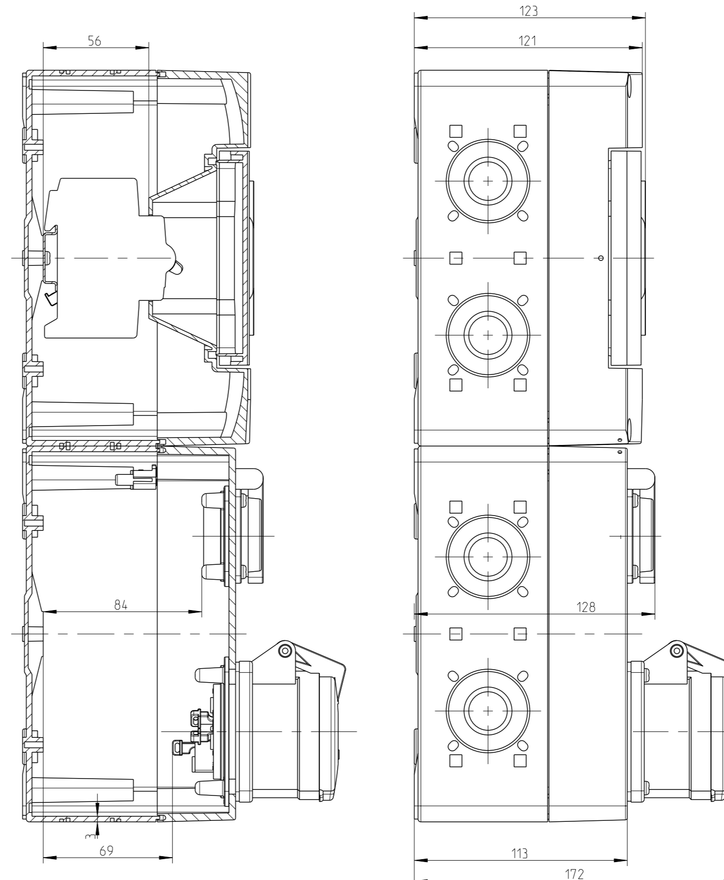
STV 912-L Innenansicht interior view
