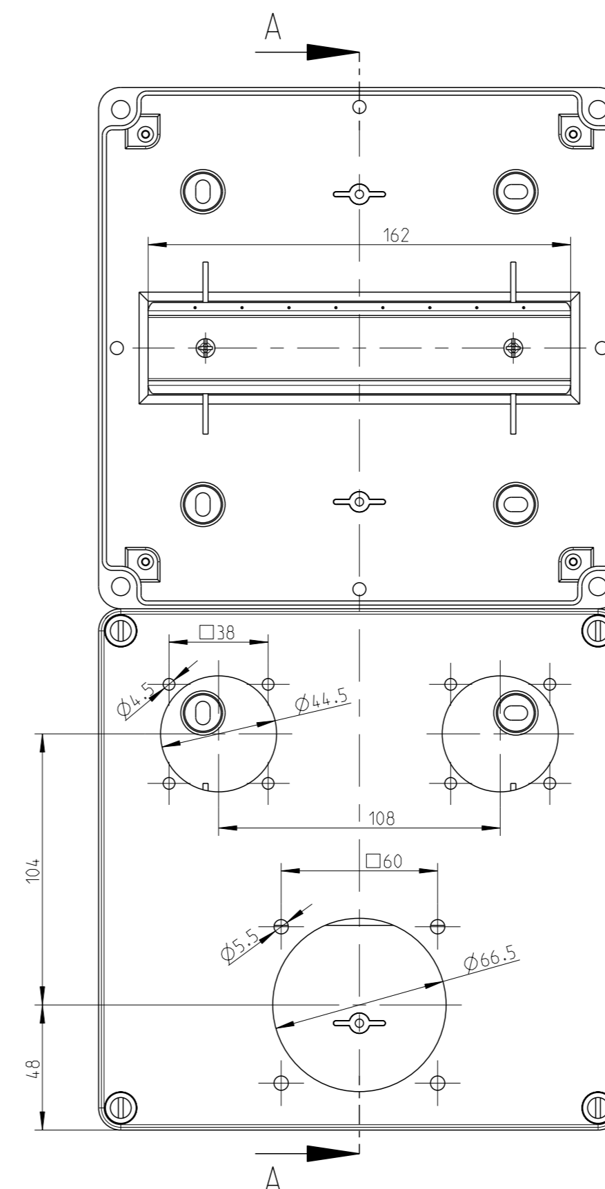
STV 912-L Innenansicht interior view
