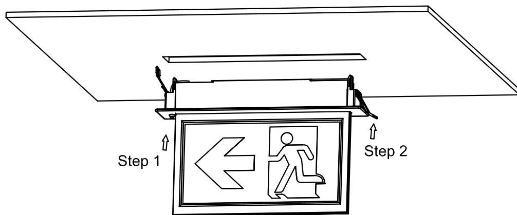
7, Rotate spring to up, press the fixture with recessed kit on mounting plate, press in one side then another.
