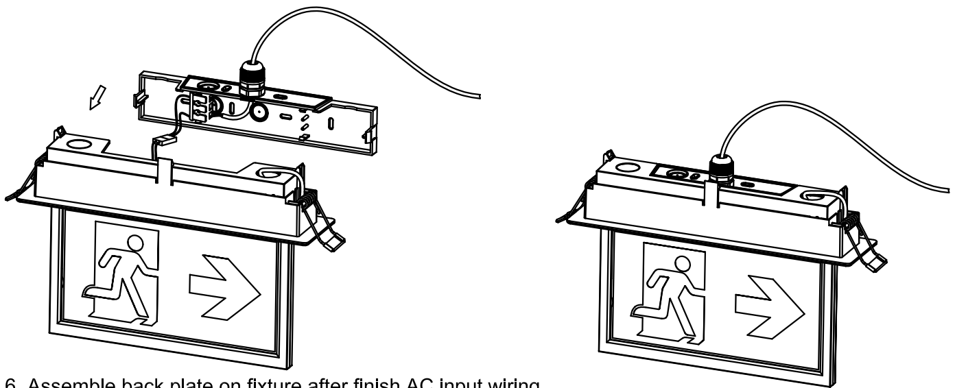
6, Assemble back plate on fixture after finish AC input wiring.
