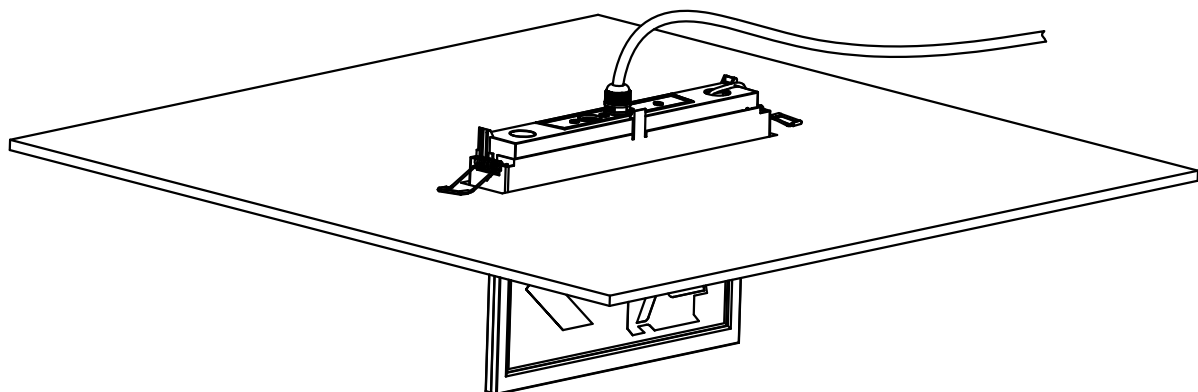
8, Finish installation.
