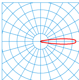
CS 19 S-MOD RE6R/3200-740 1G1 (Tube4000mm) ■ C0 - C180 TX245666 ■ C90 - C270 DIN 5040: C01 UTE: 0,51 J + 0,51 T CEN Flux Code: 1 6 27 50 101 1 6 27 50
