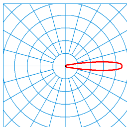
CS 19 S-MOD RE6R/2200-740 1G1 (Tube4000mm) TX245770 ■ C0 - C180 ■ C90 - C270 DIN 5040: C01 UTE: 0,51 J + 0,51 T CEN Flux Code: 1 6 27 50 101 1 6 27 50
