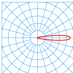
CS 19 S-MOD RE6R/4200-730 1G1 (Tube4000mm) ■ C0 - C180 TX245660 ■ C90 - C270 DIN 5040: C01 UTE: 0,51 J + 0,51 T CEN Flux Code: 1 6 27 50 101 1 6 27 50
