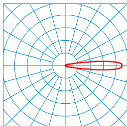
CS 19 S-MOD RE6R/3200-730 1G1 (Tube4000mm) TX245735 ■ C0 - C180 ■ C90 - C270 DIN 5040: C01 UTE: 0,51 J + 0,51 T CEN Flux Code: 1 6 27 50 101 1 6 27 50
