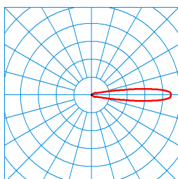
CS 19 S-MOD RE6R/4200-740 1G1 (Tube4000mm) ■ C0 - C180 TX245577 ■ C90 - C270 DIN 5040: C01 UTE: 0,51 J + 0,51 T CEN Flux Code: 1 6 27 50 101 1 6 27 50
