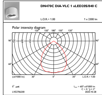
OFPC1_DN470CDIA-VLC1xLED20S840C
