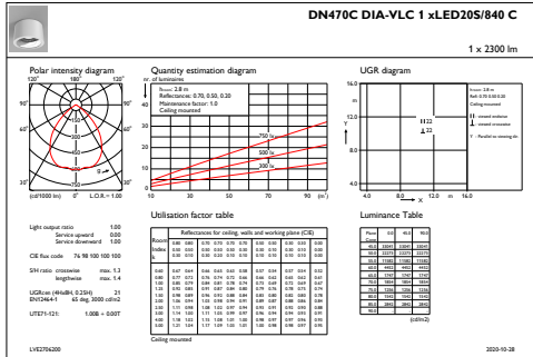
IFGU1_DN470CDIA-VLC1xLED20S840C
