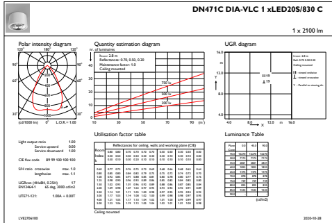
IFGU1_DN471CDIA-VLC1xLED20S830C
