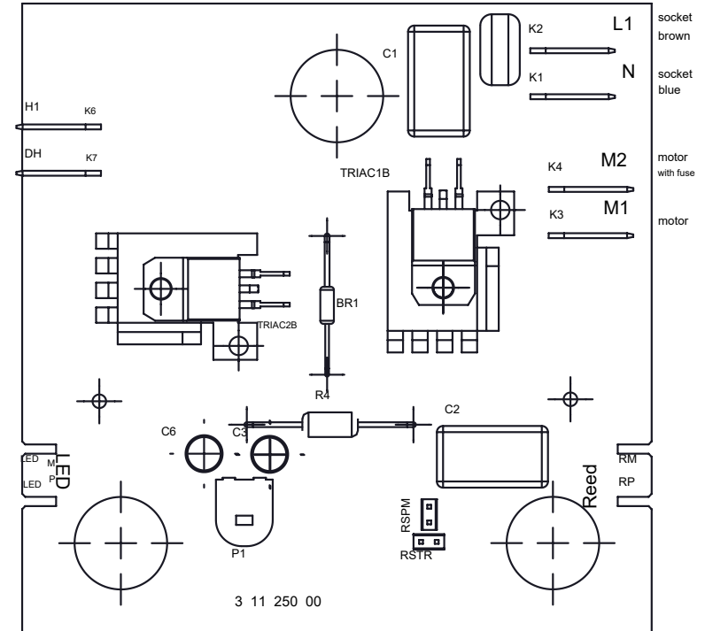
Circuit diagram electronic AirStar TB-C1
