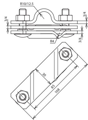
Maßbild AS S TE 25 7.10 FL40 STTZN
