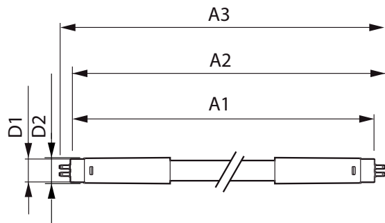
MAS LEDtube 600mm HE 8W 840 T5
