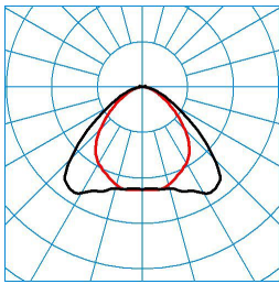
ELINE FL HE LVW120 865 L150 1 20
