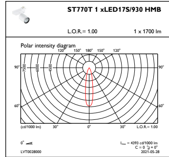
OFPC1_ST770T1xLED17S930HMB
