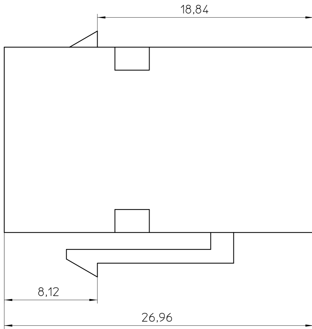
Panel cut out
