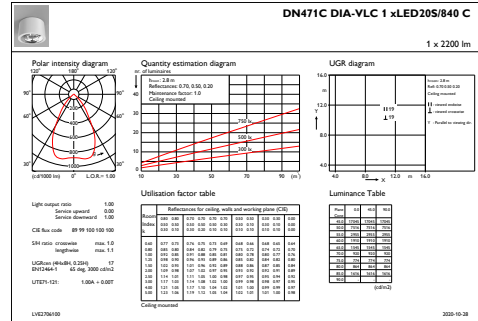
IFGU1_DN471CDIA-VLC1xLED20S840C
