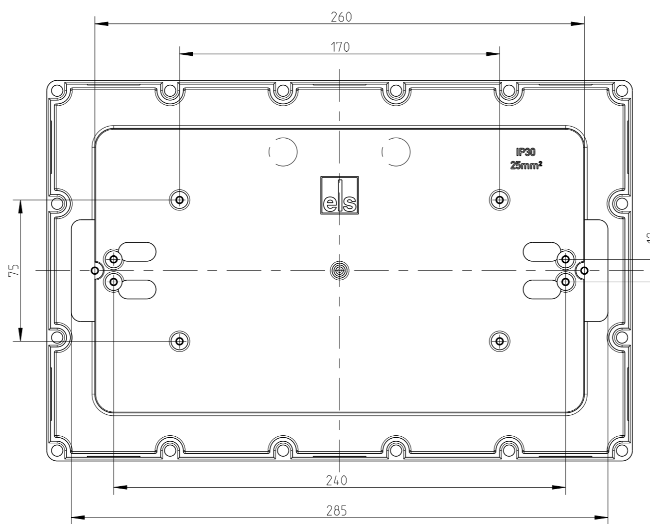
Innenansicht Boden / interior view ground
