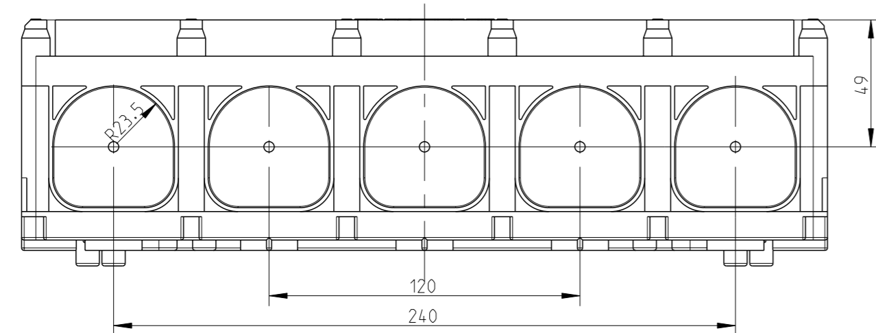
Innenansicht Kasten / interior view of the box
