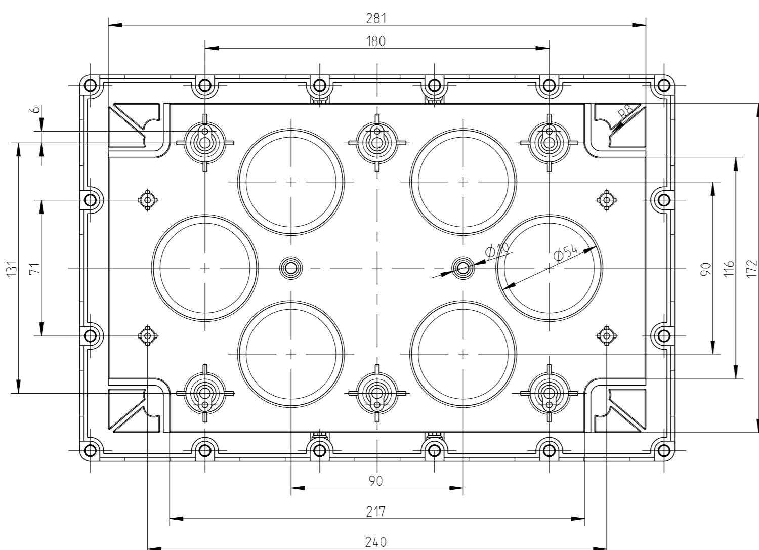
Innenansicht Kasten / interior view of the box
