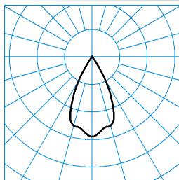
SncPoint 905 C02 BR-FL LED1100-830 01 ■ C0 - C180 TX047927
