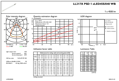
IFGU1_LL217XPSD1xLED45S840WB
