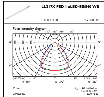
OFPC1_LL217XPSD1xLED45S840WB
