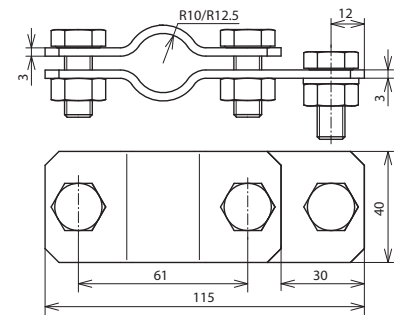
Maßbild AS TE 25 ASSM10 STTZN
