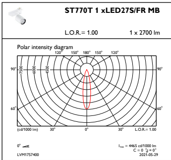
OFPC1_ST770T1xLED27SFRMB
