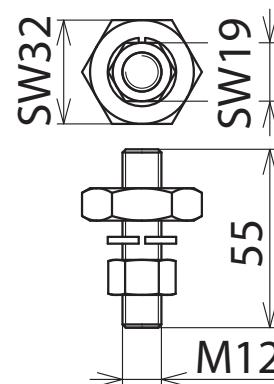
Maßbild AS SCHR M12 55
