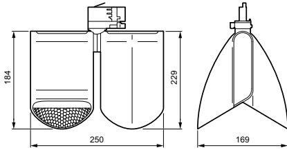
ST762T 27S/830 DIA BK
