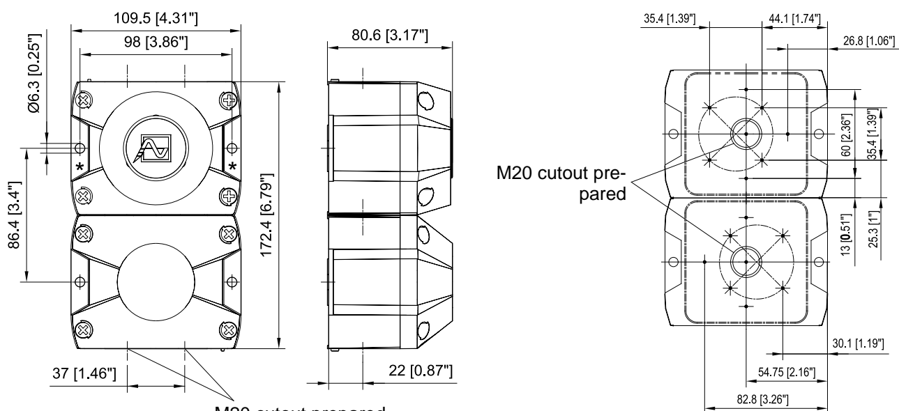
Drilling pattern inside the housing
