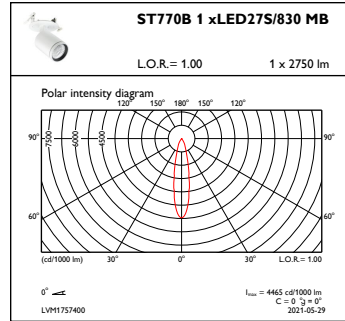
OFPC1_ST770B1xLED27S830MB
