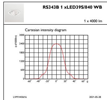
IFCC1_RS343B1xLED39S840WB
