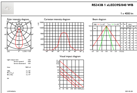
IFAS1_RS343B1xLED39S840WB
