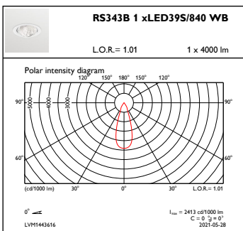
OFPC1_RS343B1xLED39S840WB
