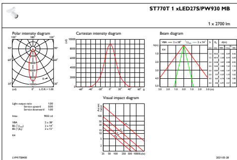
IFAS1_ST770T1xLED27SPW930MB
