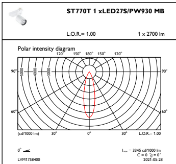
OFPC1_ST770T1xLED27SPW930MB
