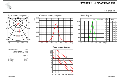
IFAS1_ST780T1xLED60S840MB
