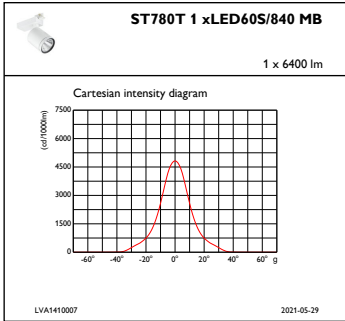
IFCC1_ST780T1xLED60S840MB
