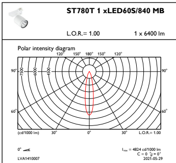
OFPC1_ST780T1xLED60S840MB
