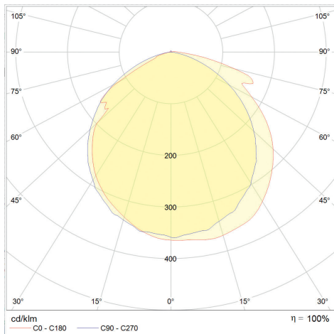
EL-500, 2.700 K, R_a > 90
