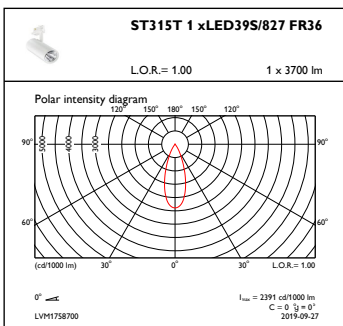
OFPC1_ST315T1xLED39S827FR36
