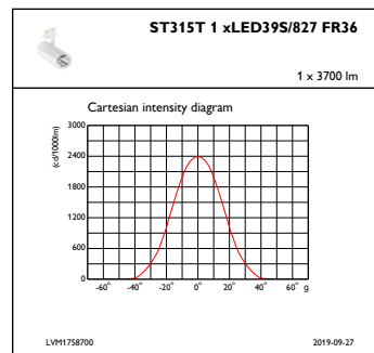
IFCC1_ST315T1xLED39S827FR36
