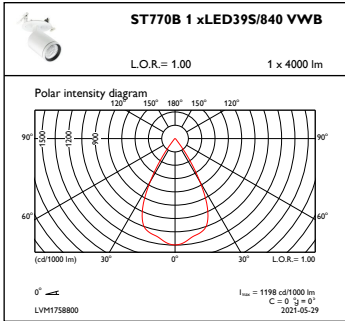
OFPC1_ST770B1xLED39S840VWB
