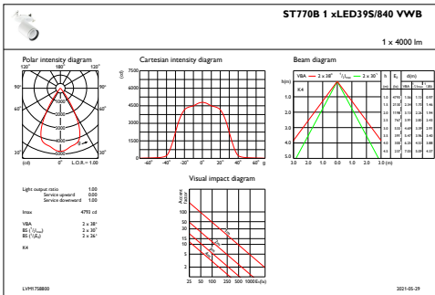
IFAS1_ST770B1xLED39S840VWB
