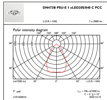
OFPC1_DN473BPSU-E1xLED20S840CPCC
