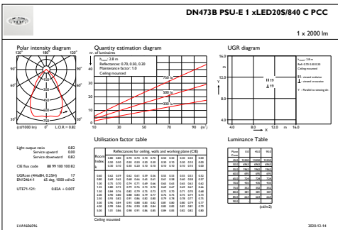
IFGU1_DN473BPSU-E1xLED20S840CPCC
