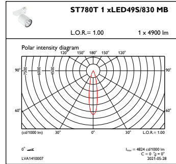
OFPC1_ST780T1xLED49S830MB
