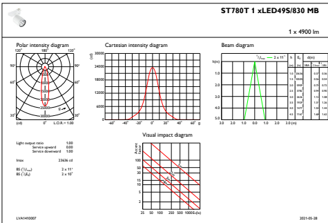
IFAS1_ST780T1xLED49S830MB
