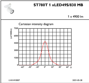
IFCC1_ST780T1xLED49S830MB
